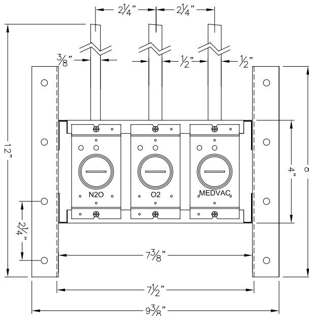
Triple Outlet
