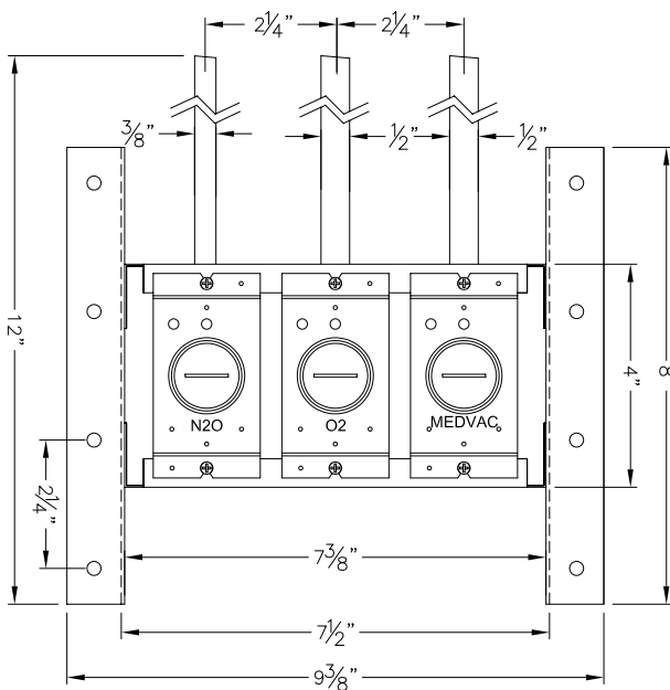
Triple Outlet
