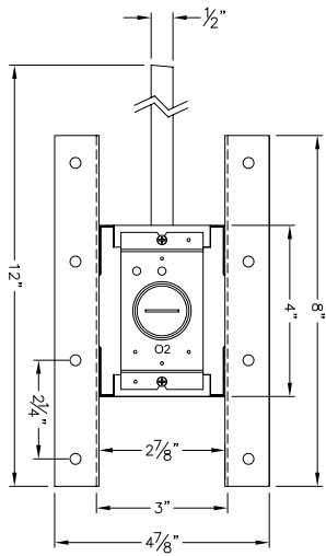
Single Outlet
